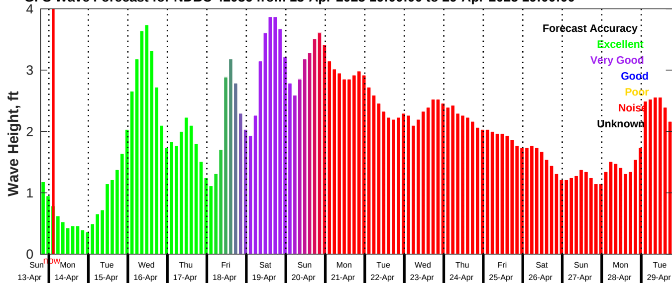
GFS Wave Forecast for NDBC 42036 from 13-Apr-2025 19:00:00 to 29-Apr-2025 19:00:00
