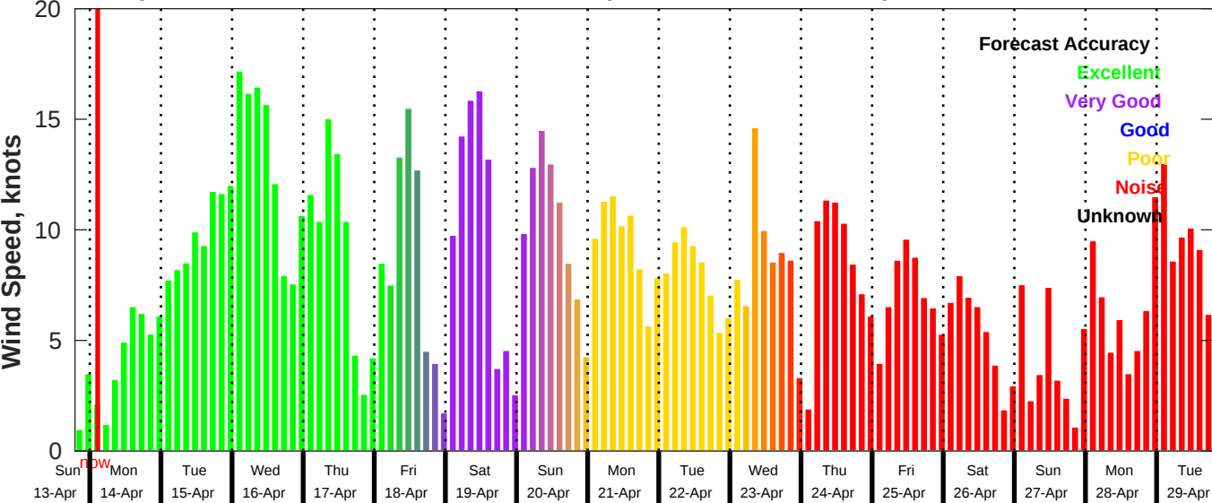
GFS Wind Speed Forecast for NDBC 42036 from 13-Apr-2025 19:00:00 to 29-Apr-2025 19:00:00
