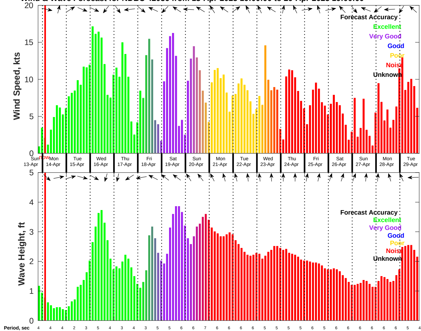
Wind & Wave Forecast for NDBC 42036 from 13-Apr-2025 19:00:00 to 29-Apr-2025 19:00:00
