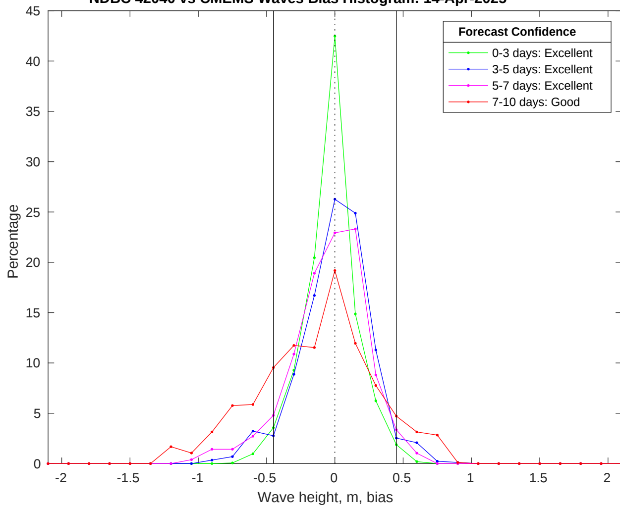
NDBC 42040 vs CMEMS Waves Bias Histogram: 14-Apr-2025
