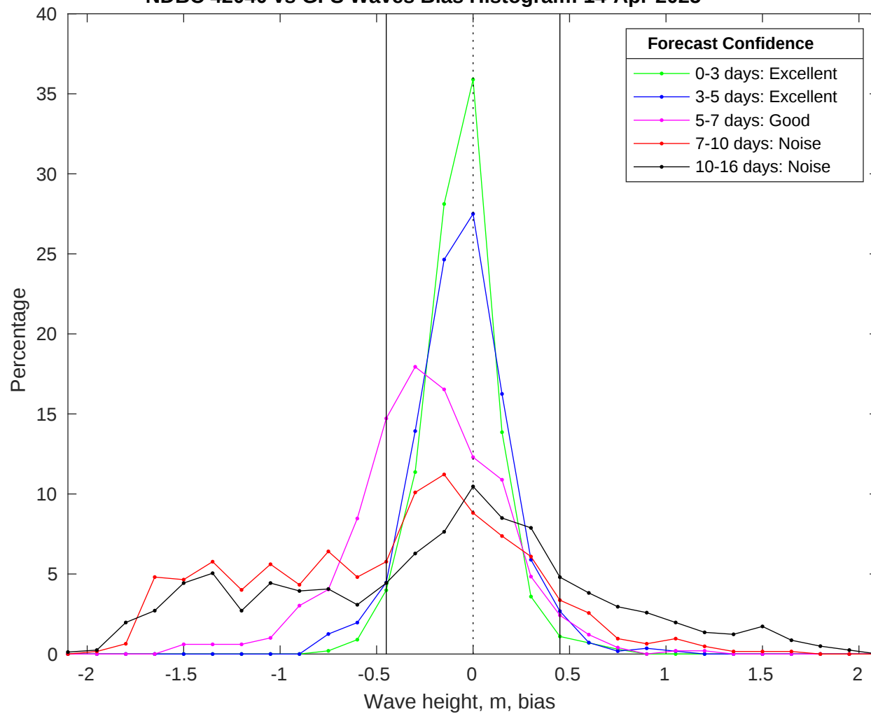
NDBC 42040 vs GFS Waves Bias Histogram: 14-Apr-2025
