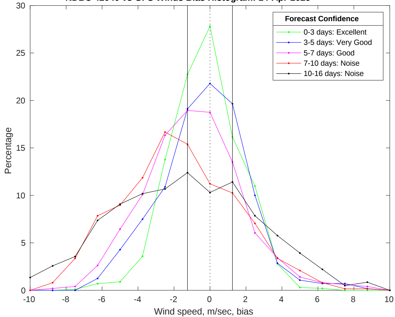
NDBC 42040 vs GFS Winds Bias Histogram: 14-Apr-2025
