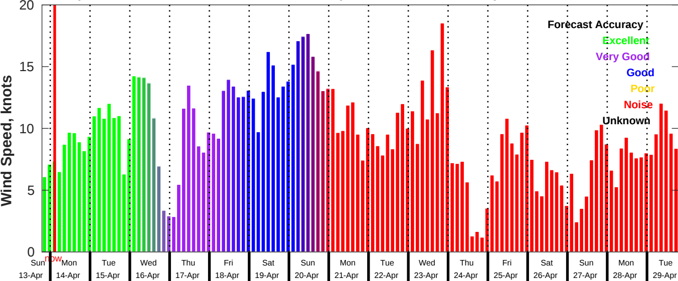
GFS Wind Speed Forecast for NDBC 42040 from 13-Apr-2025 19:00:00 to 29-Apr-2025 19:00:00
