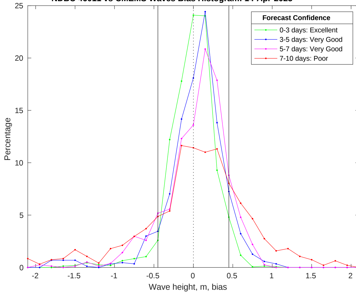
NDBC 46011 vs CMEMS Waves Bias Histogram: 14-Apr-2025
