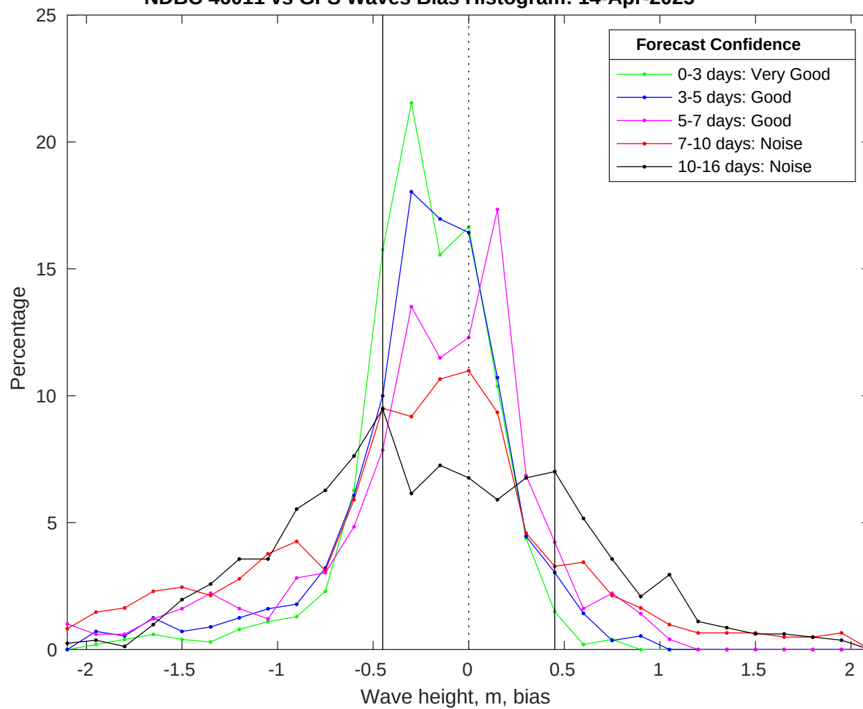
NDBC 46011 vs GFS Waves Bias Histogram: 14-Apr-2025
