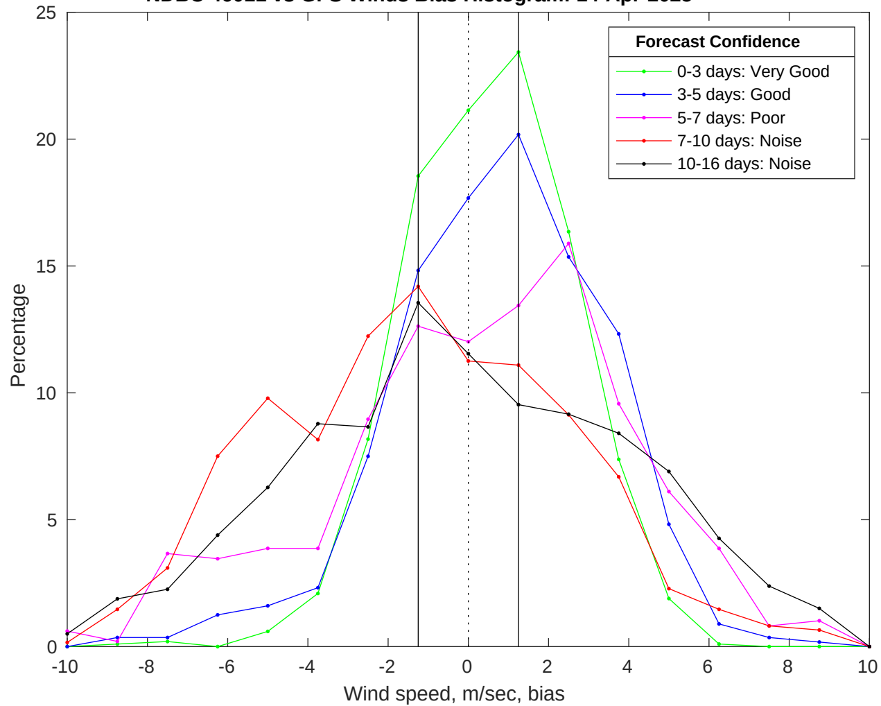
NDBC 46011 vs GFS Winds Bias Histogram: 14-Apr-2025
