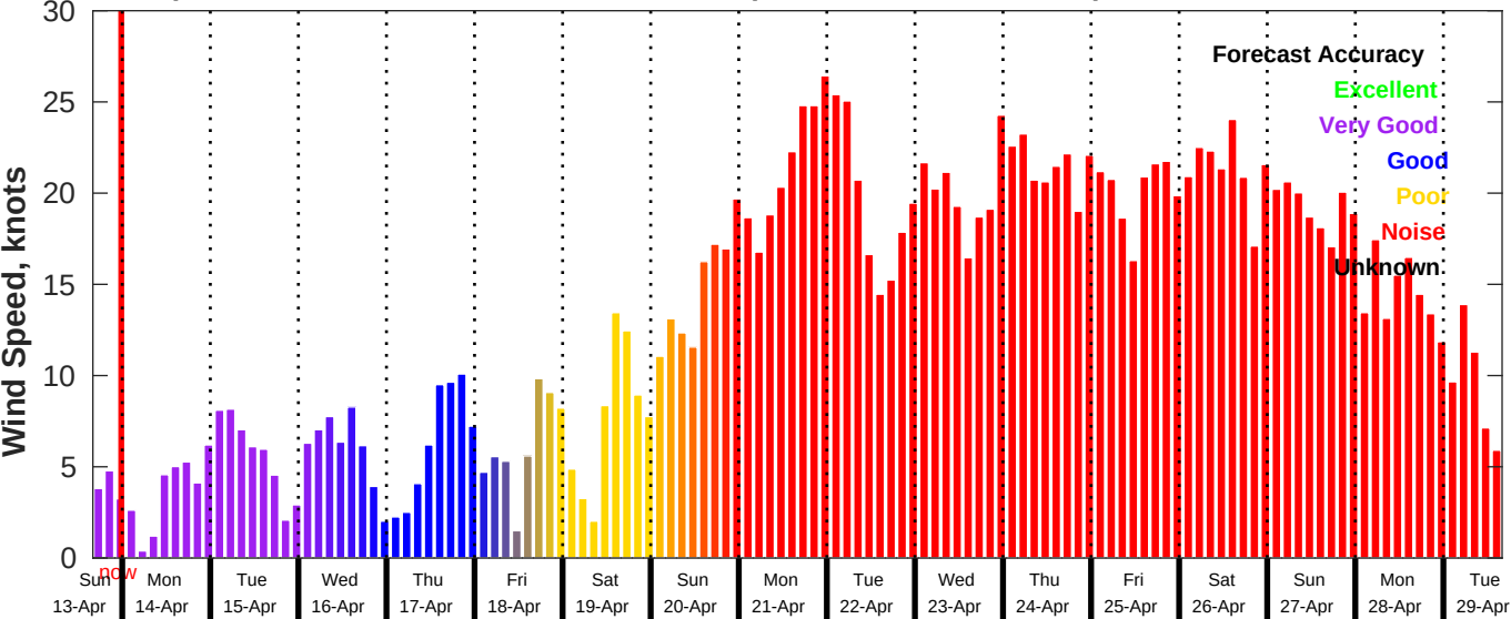
GFS Wind Speed Forecast for NDBC 46011 from 13-Apr-2025 16:00:00 to 29-Apr-2025 16:00:00
