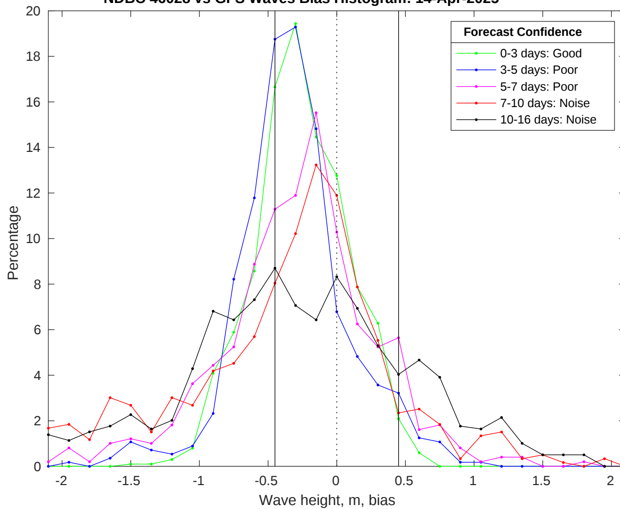
NDBC 46028 vs GFS Waves Bias Histogram: 14-Apr-2025
