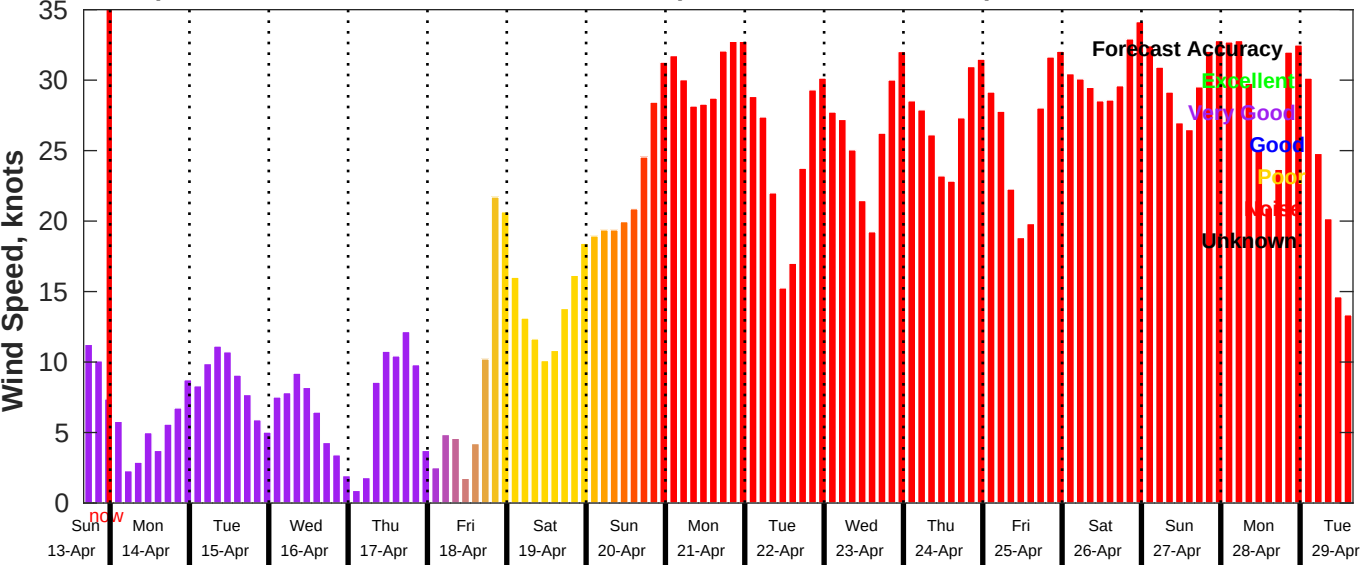
GFS Wind Speed Forecast for NDBC 46028 from 13-Apr-2025 16:00:00 to 29-Apr-2025 16:00:00
