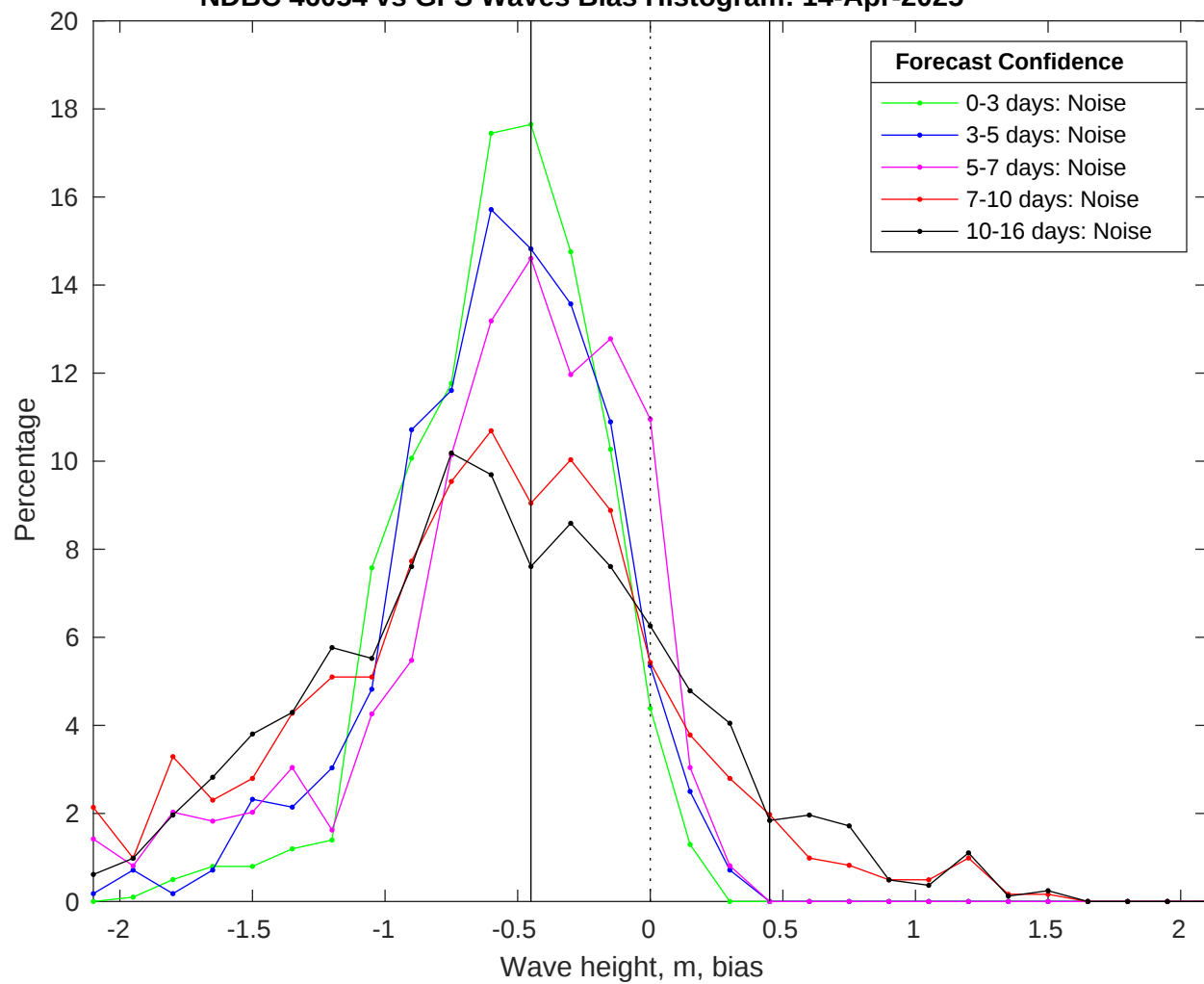
NDBC 46054 vs GFS Waves Bias Histogram: 14-Apr-2025
