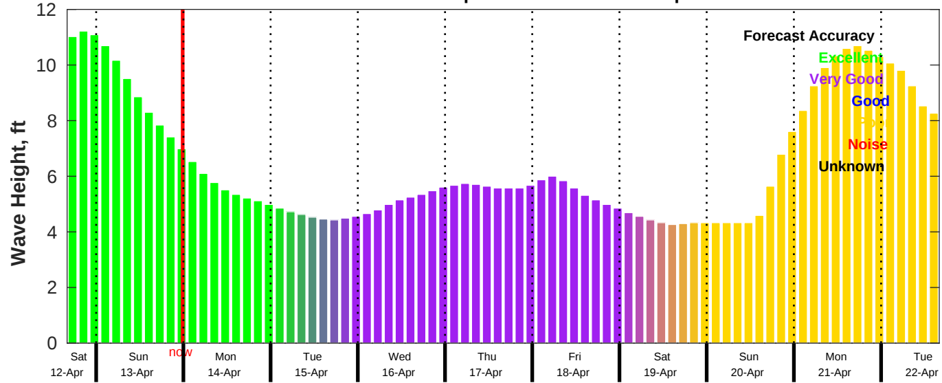
CMEMS Wave Forecast for NDBC 46054 from 12-Apr-2025 16:00:00 to 22-Apr-2025 16:00:00
