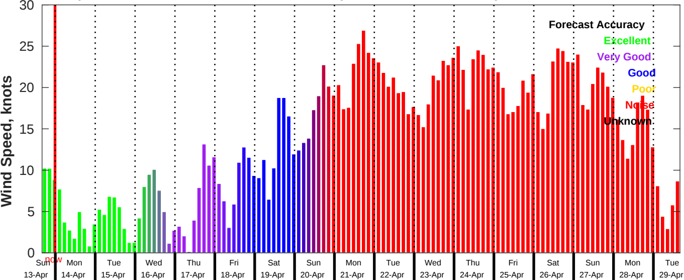
GFS Wind Speed Forecast for NDBC 46054 from 13-Apr-2025 16:00:00 to 29-Apr-2025 16:00:00
