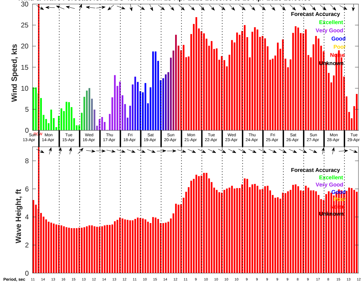
Wind & Wave Forecast for NDBC 46054 from 13-Apr-2025 16:00:00 to 29-Apr-2025 16:00:00
