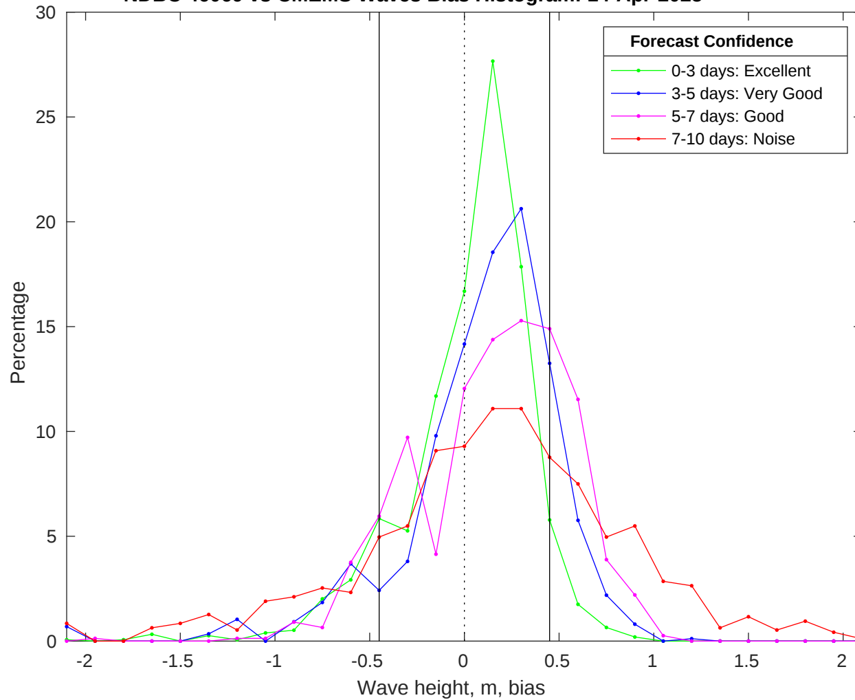
NDBC 46069 vs CMEMS Waves Bias Histogram: 14-Apr-2025
