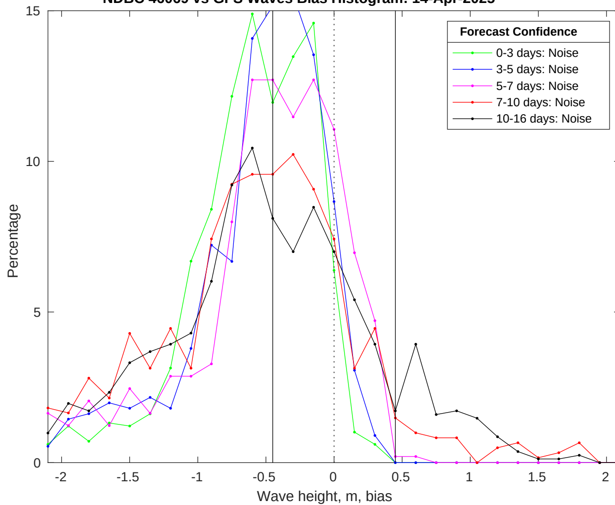
NDBC 46069 vs GFS Waves Bias Histogram: 14-Apr-2025
