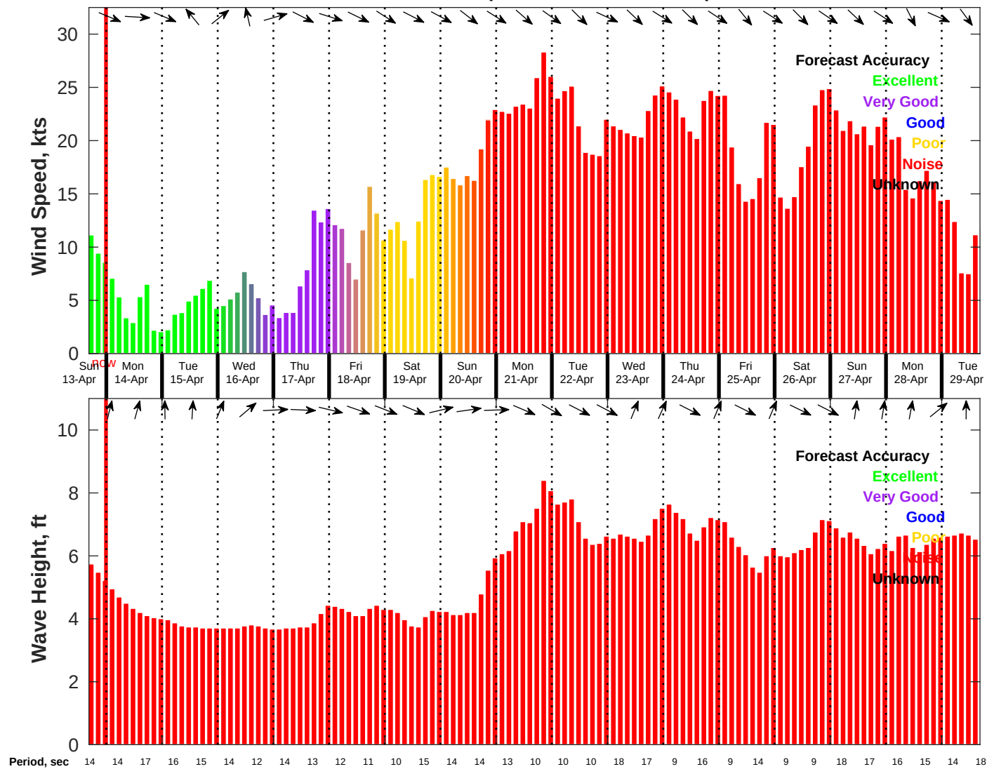
Wind & Wave Forecast for NDBC 46069 from 13-Apr-2025 16:00:00 to 29-Apr-2025 16:00:00
