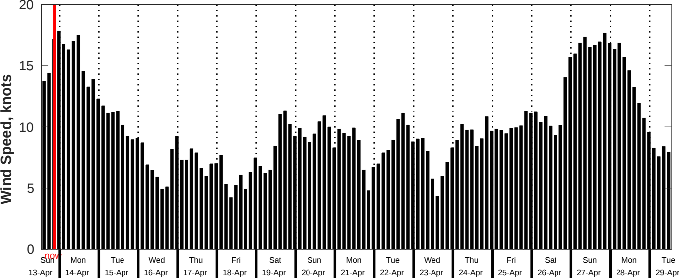
GFS Wind Speed Forecast for NDBC 51209 from 13-Apr-2025 13:00:00 to 29-Apr-2025 13:00:00
