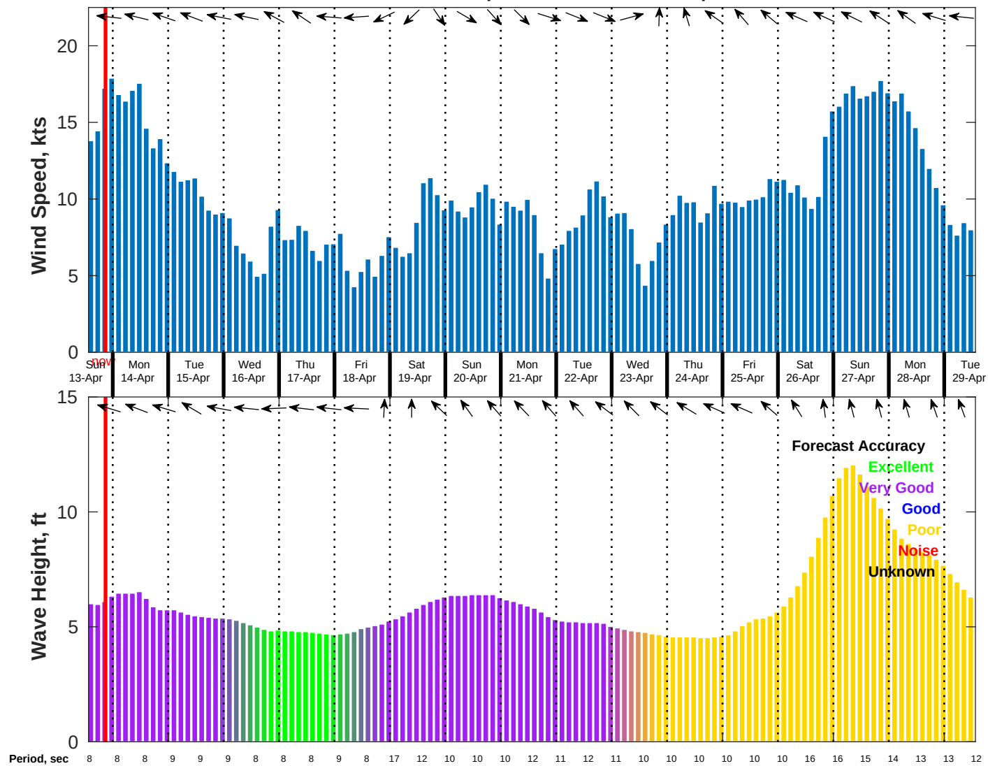
Wind & Wave Forecast for NDBC 51209 from 13-Apr-2025 13:00:00 to 29-Apr-2025 13:00:00
