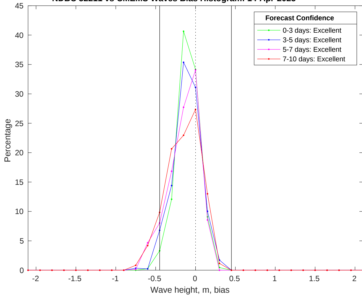
NDBC 52211 vs CMEMS Waves Bias Histogram: 14-Apr-2025
