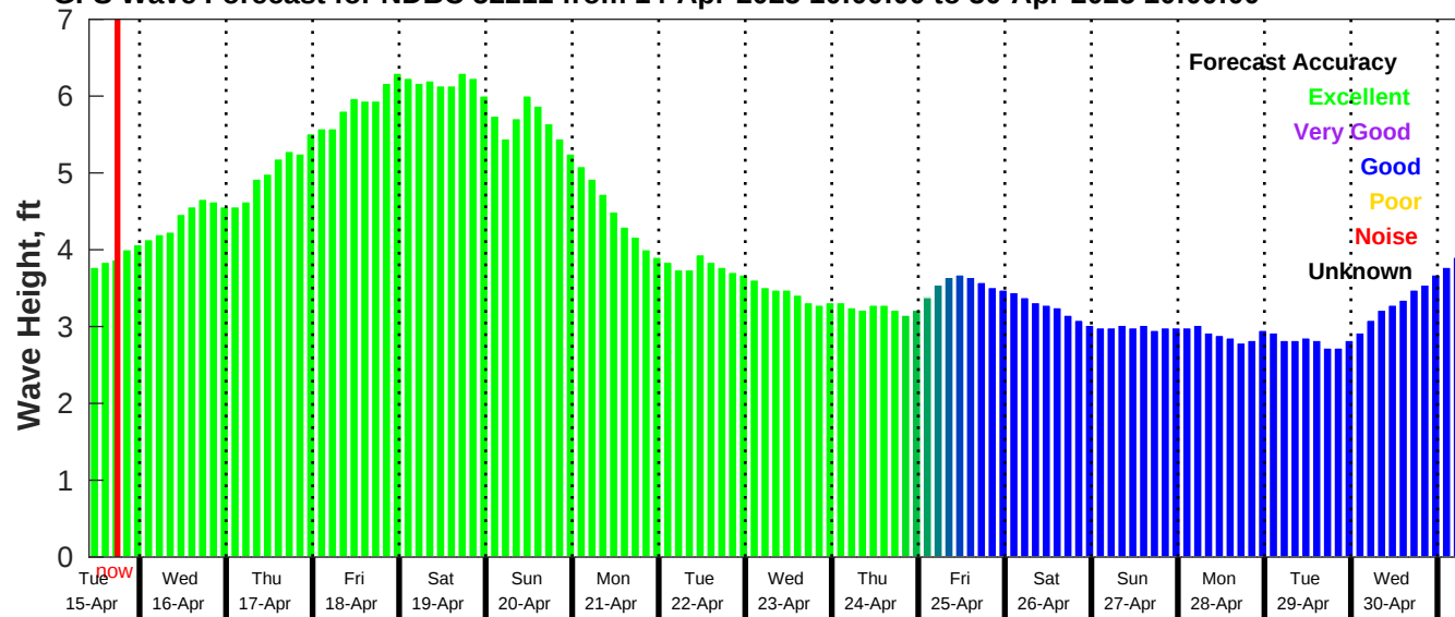
GFS Wave Forecast for NDBC 52211 from 14-Apr-2025 10:00:00 to 30-Apr-2025 10:00:00
