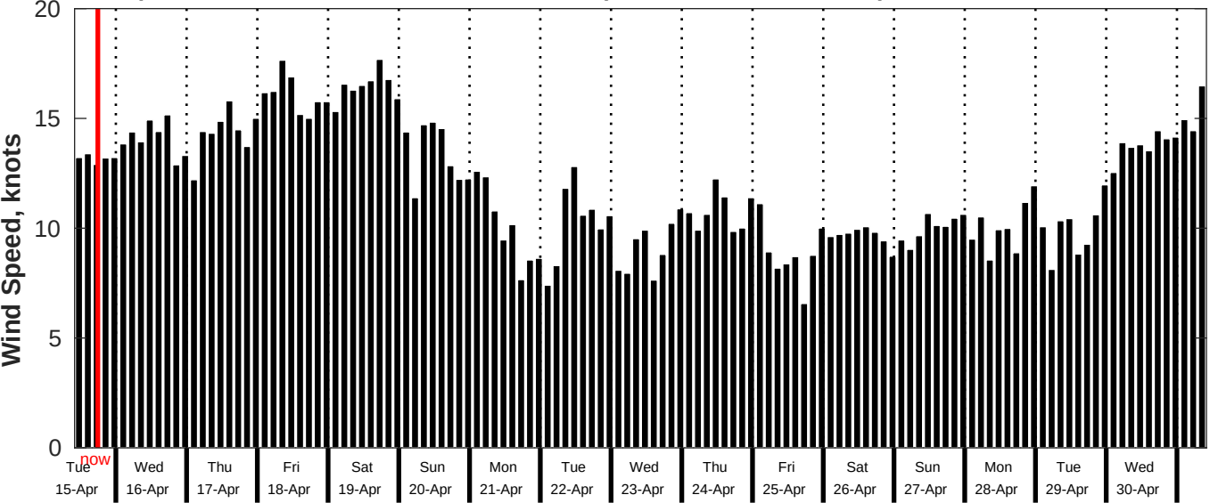
GFS Wind Speed Forecast for NDBC 52211 from 14-Apr-2025 10:00:00 to 30-Apr-2025 10:00:00
