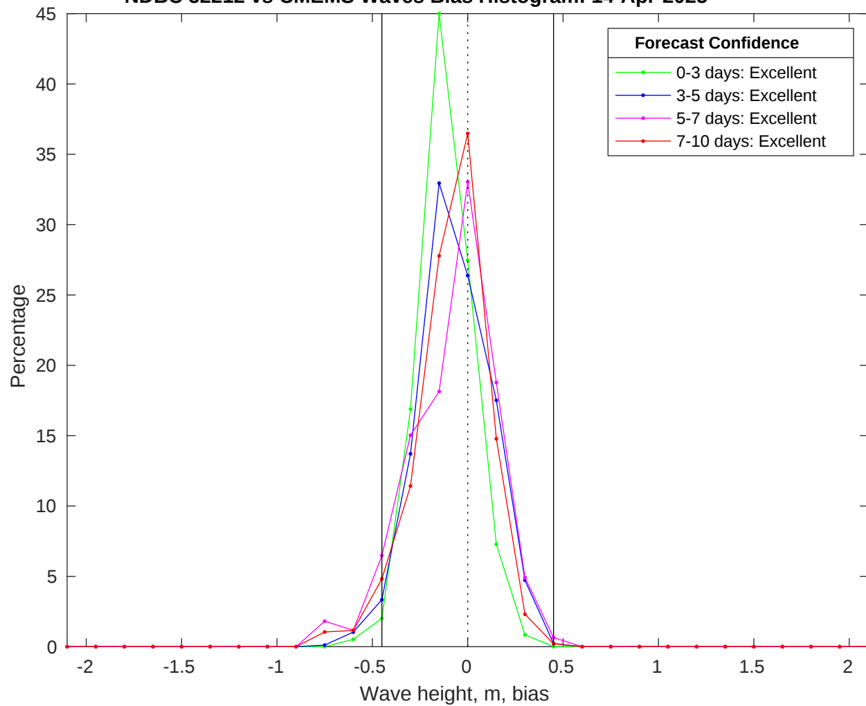
NDBC 52212 vs CMEMS Waves Bias Histogram: 14-Apr-2025
