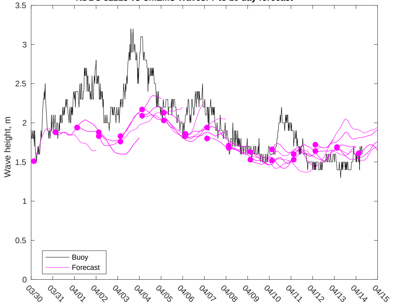
NDBC 52213 vs CMEMS Waves: 7 to 10 day forecast
