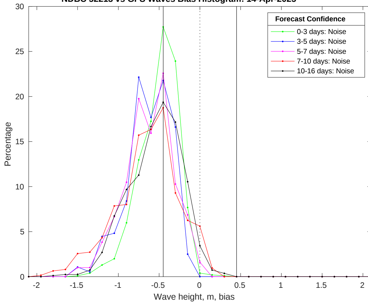
NDBC 52213 vs GFS Waves Bias Histogram: 14-Apr-2025
