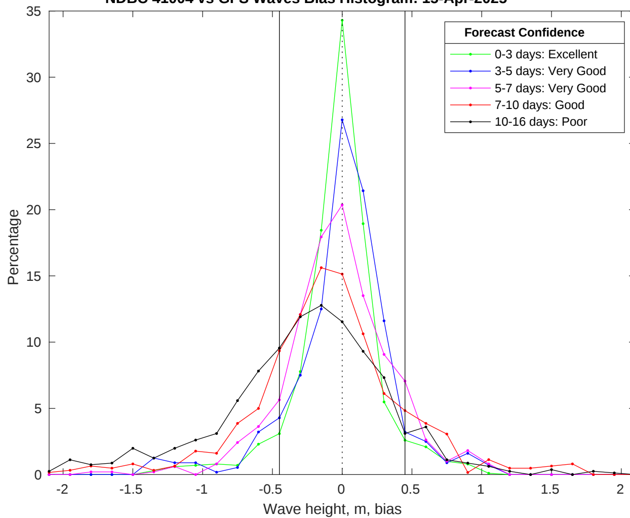
NDBC 41004 vs GFS Waves Bias Histogram: 15-Apr-2025
