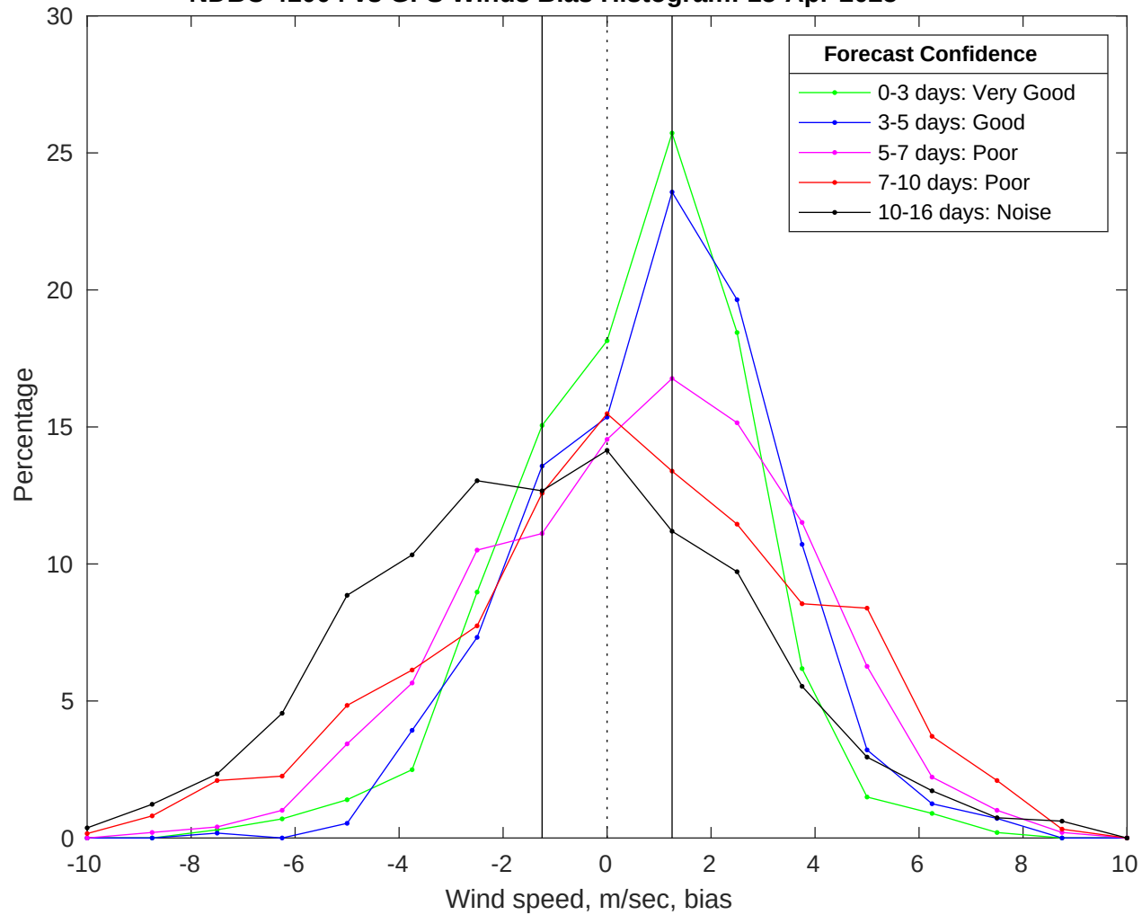
NDBC 41004 vs GFS Winds Bias Histogram: 15-Apr-2025
