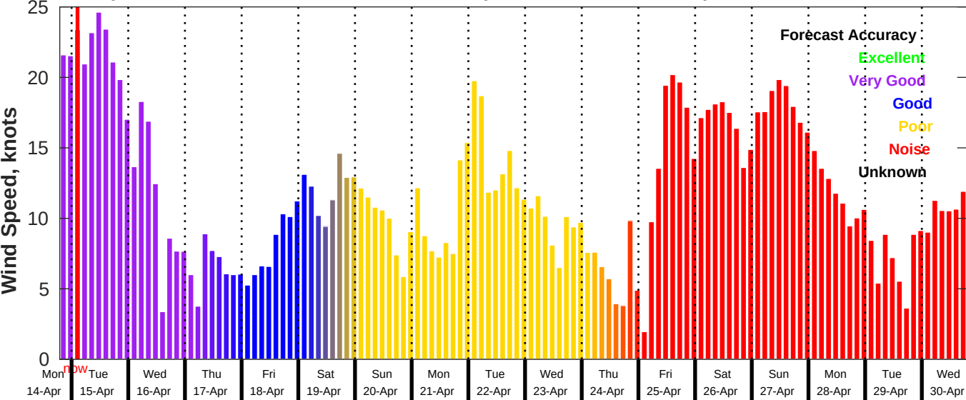
GFS Wind Speed Forecast for NDBC 41004 from 14-Apr-2025 19:00:00 to 30-Apr-2025 19:00:00
