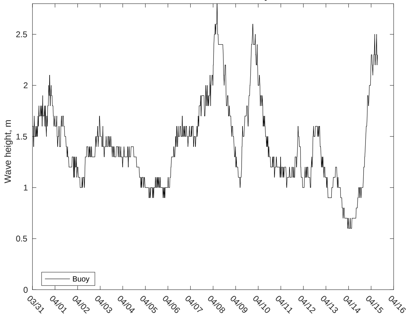
NDBC 41013 vs CMEMS Waves: 10 to 16 day forecast
