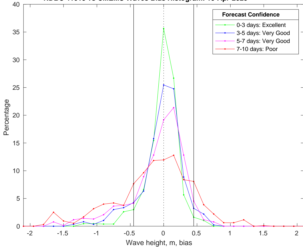
NDBC 41013 vs CMEMS Waves Bias Histogram: 15-Apr-2025
