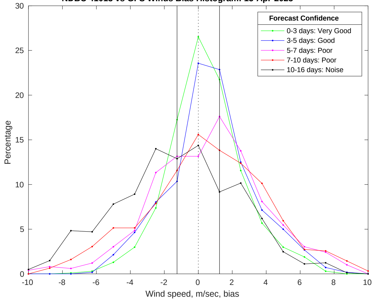
NDBC 41013 vs GFS Winds Bias Histogram: 15-Apr-2025
