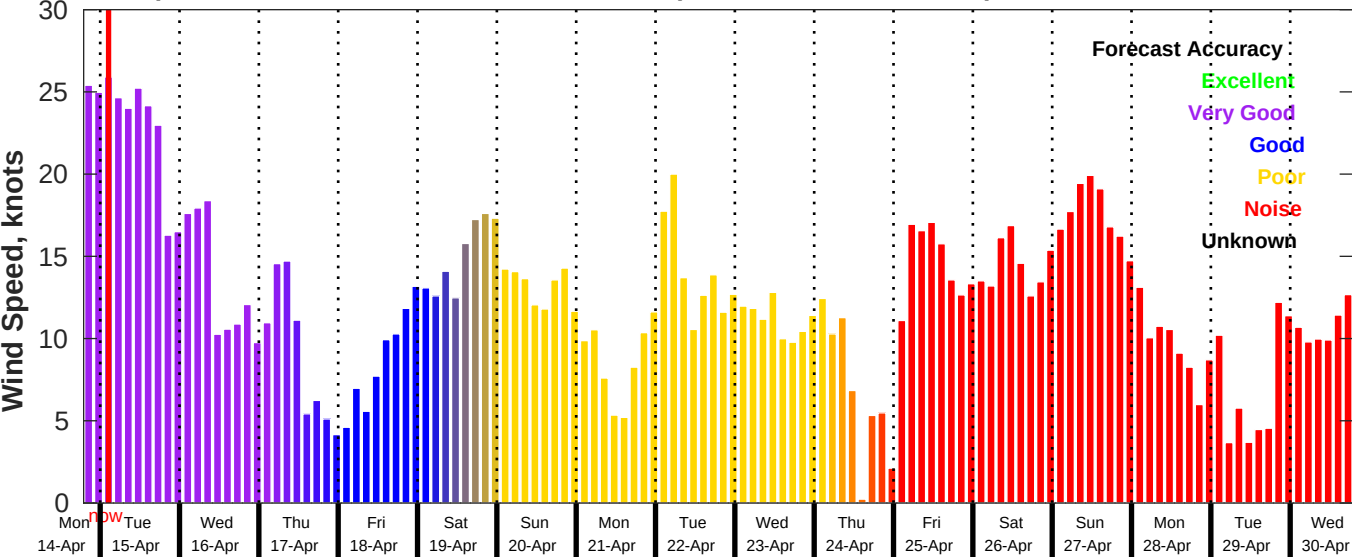
GFS Wind Speed Forecast for NDBC 41013 from 14-Apr-2025 19:00:00 to 30-Apr-2025 19:00:00
