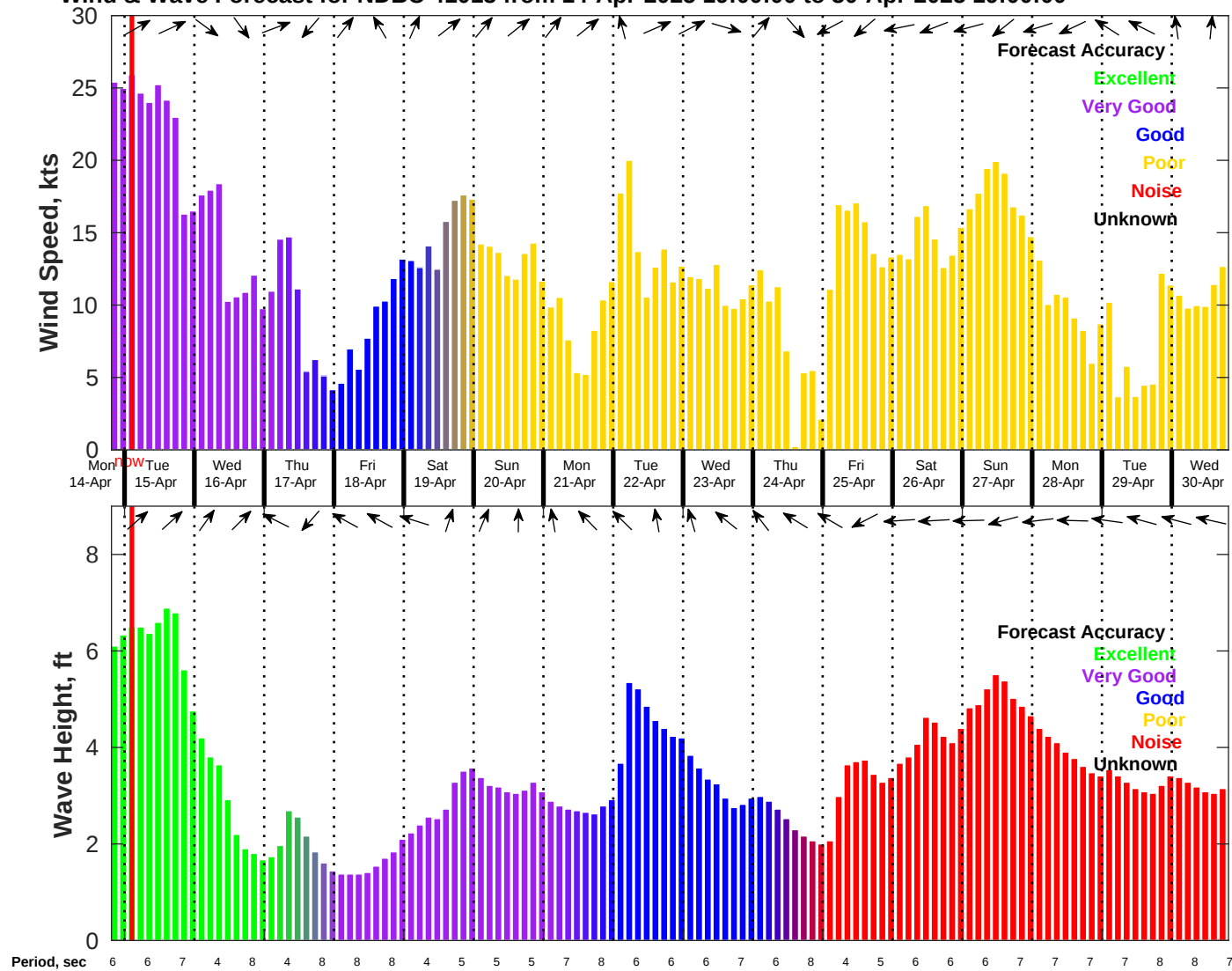
Wind & Wave Forecast for NDBC 41013 from 14-Apr-2025 19:00:00 to 30-Apr-2025 19:00:00
