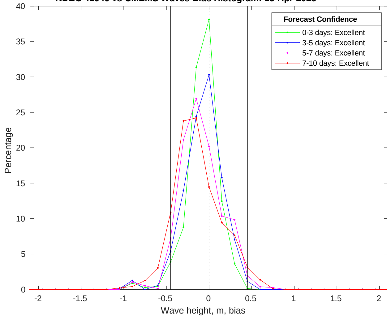
NDBC 41040 vs CMEMS Waves Bias Histogram: 15-Apr-2025
