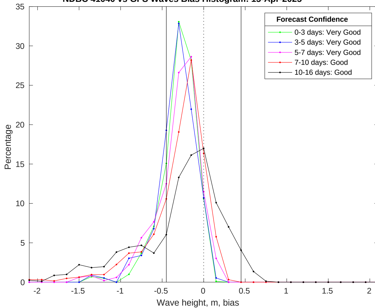
NDBC 41040 vs GFS Waves Bias Histogram: 15-Apr-2025
