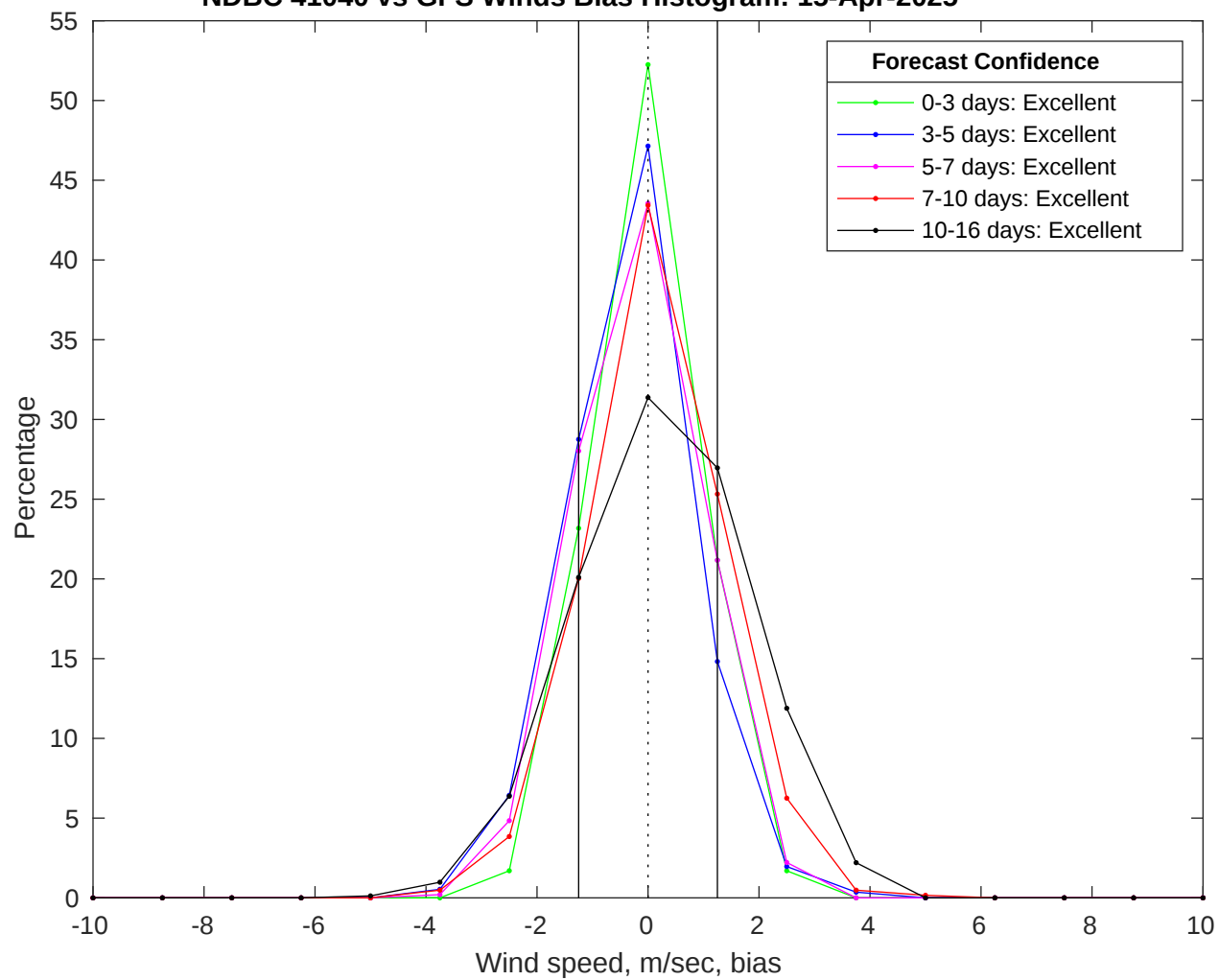
NDBC 41040 vs GFS Winds Bias Histogram: 15-Apr-2025
