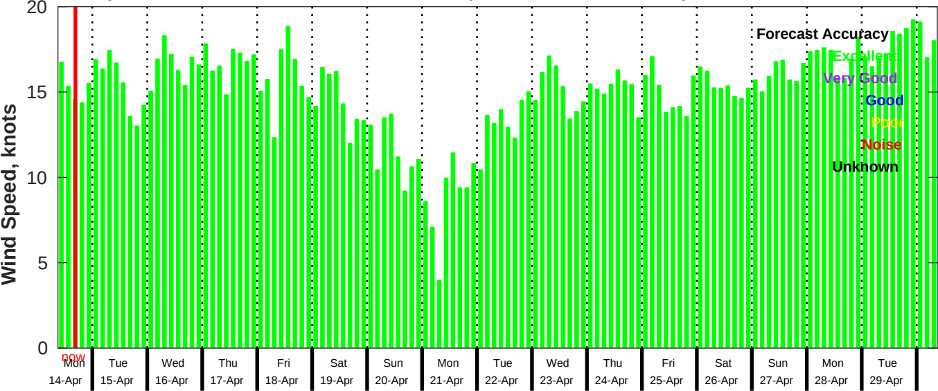
GFS Wind Speed Forecast for NDBC 41040 from 14-Apr-2025 09:00:00 to 30-Apr-2025 09:00:00
