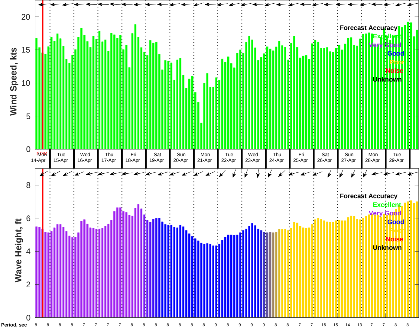
Wind & Wave Forecast for NDBC 41040 from 14-Apr-2025 09:00:00 to 30-Apr-2025 09:00:00
