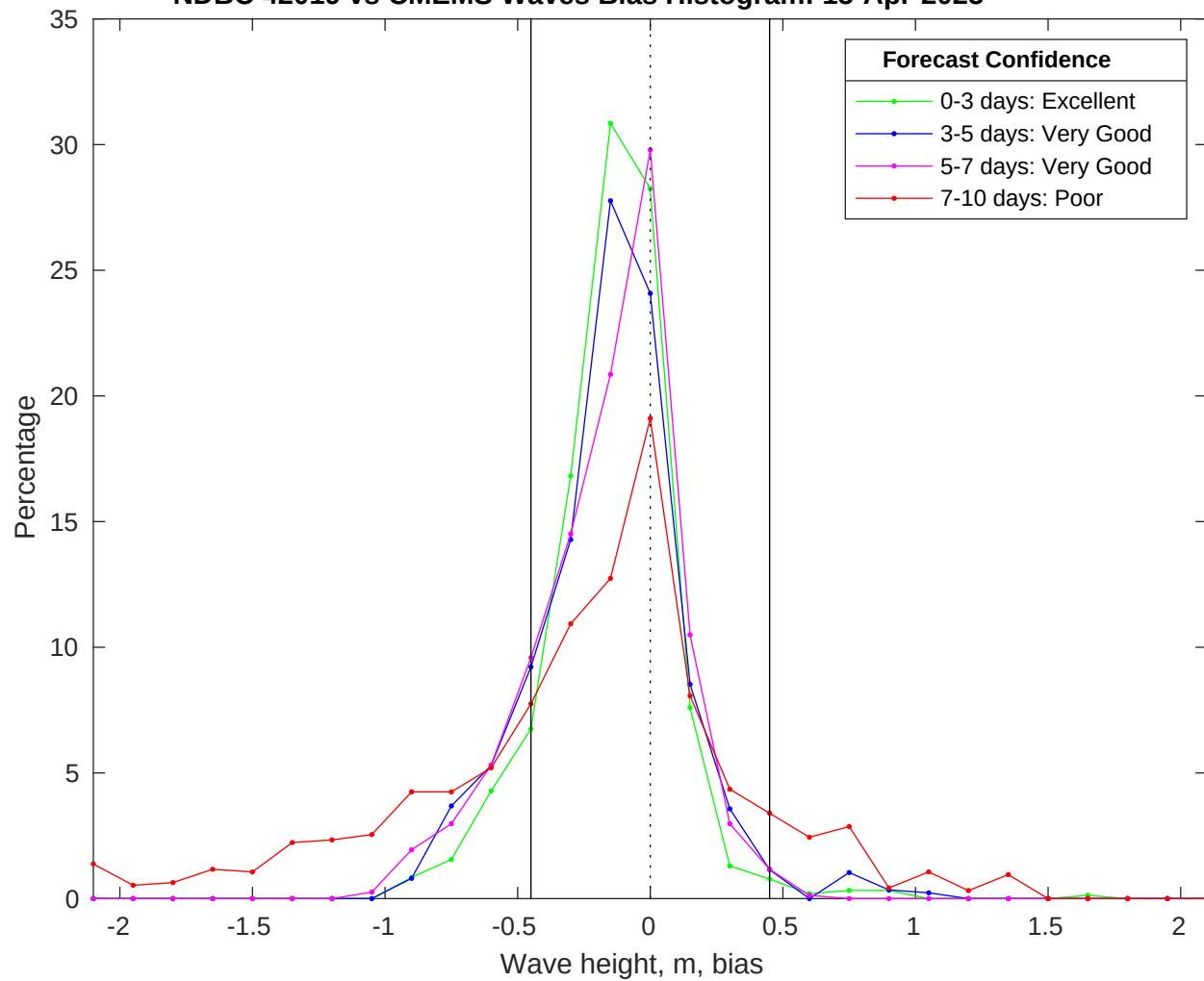
NDBC 42019 vs CMEMS Waves Bias Histogram: 15-Apr-2025
