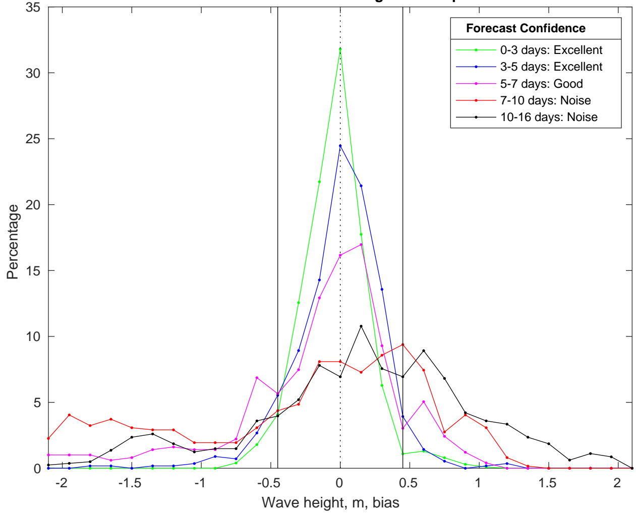
NDBC 42019 vs GFS Waves Bias Histogram: 15-Apr-2025
