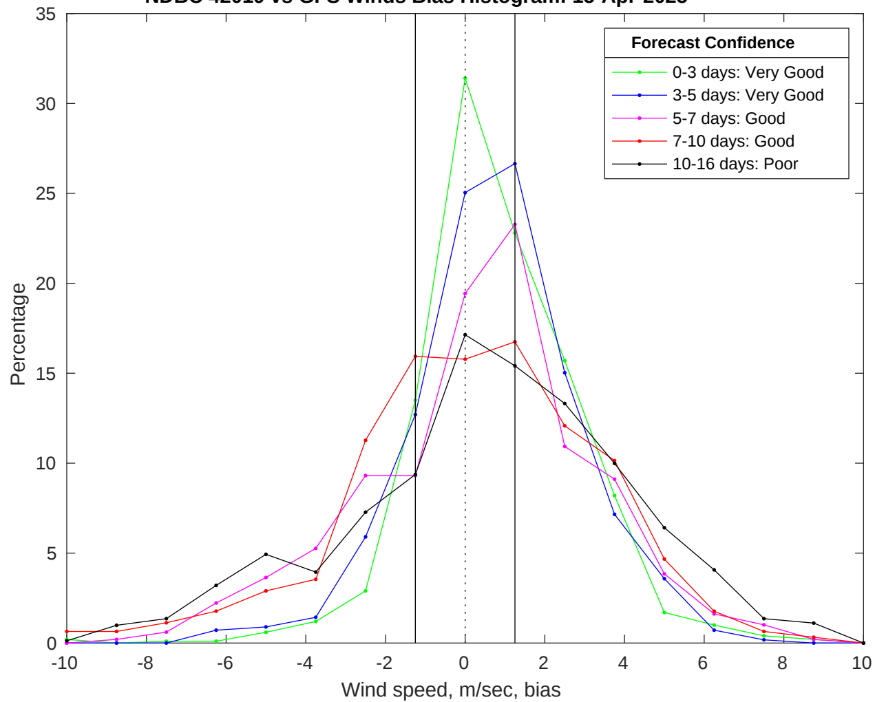
NDBC 42019 vs GFS Winds Bias Histogram: 15-Apr-2025
