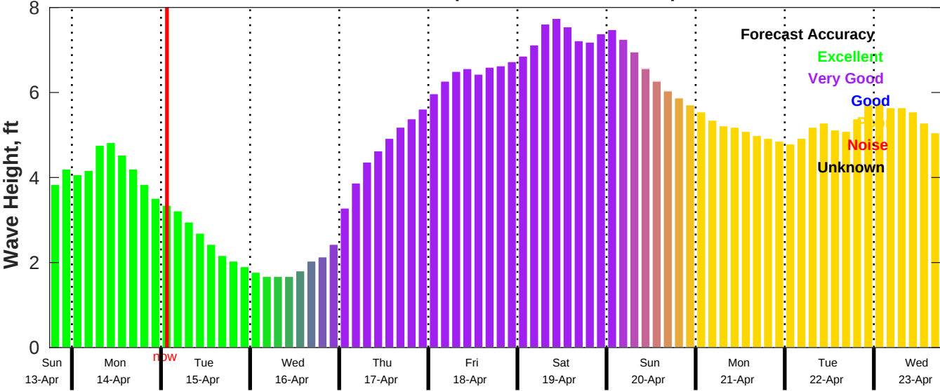
CMEMS Wave Forecast for NDBC 42019 from 13-Apr-2025 18:00:00 to 23-Apr-2025 18:00:00
