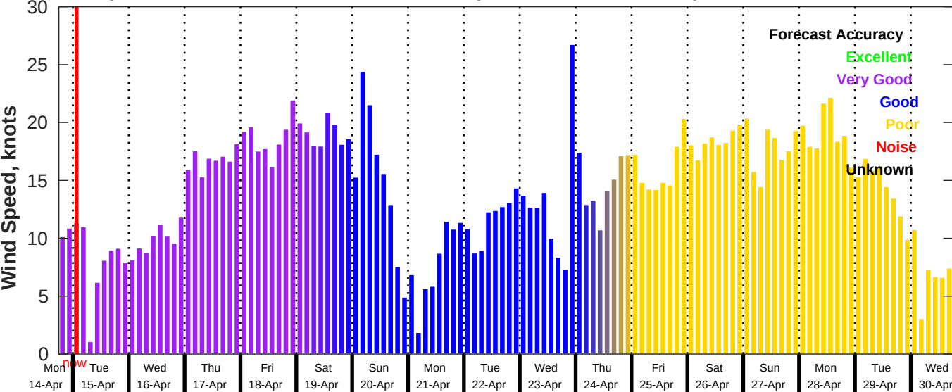
GFS Wind Speed Forecast for NDBC 42019 from 14-Apr-2025 18:00:00 to 30-Apr-2025 18:00:00
