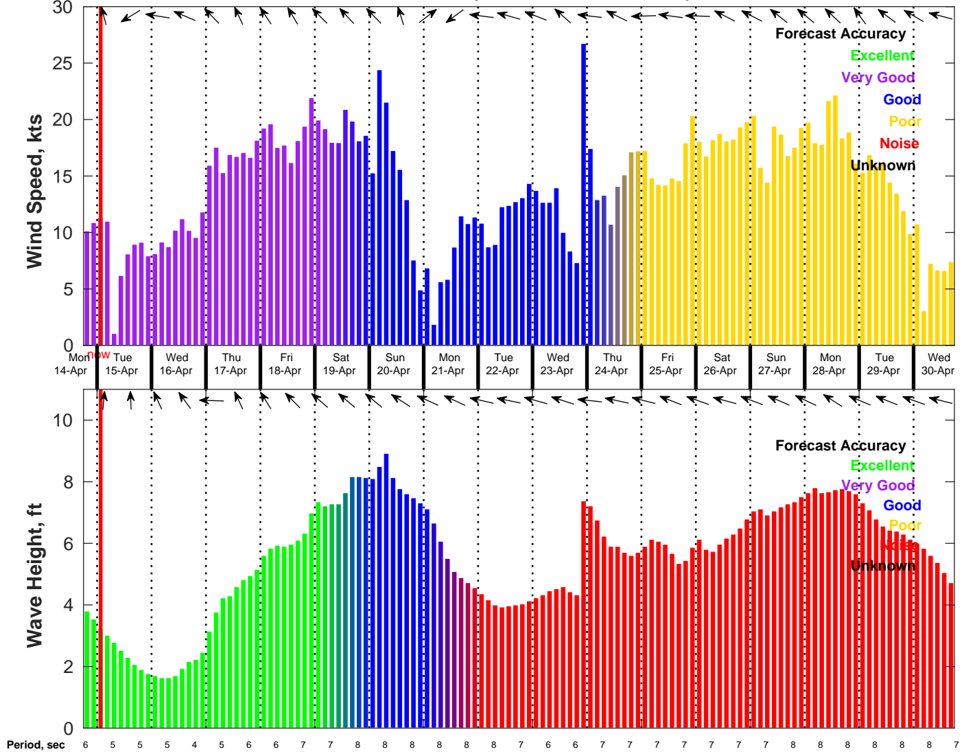
Wind & Wave Forecast for NDBC 42019 from 14-Apr-2025 18:00:00 to 30-Apr-2025 18:00:00
