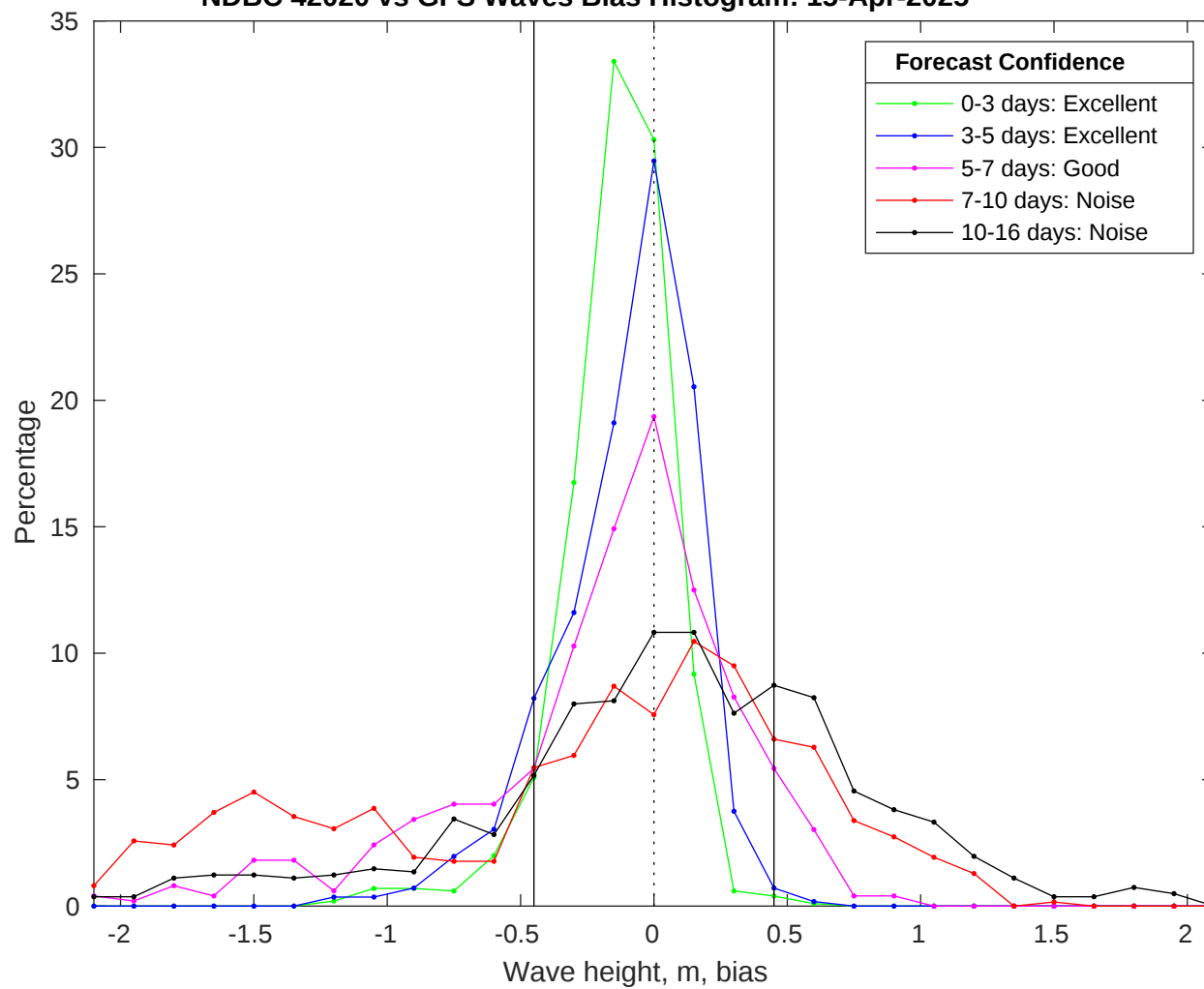
NDBC 42020 vs GFS Waves Bias Histogram: 15-Apr-2025
