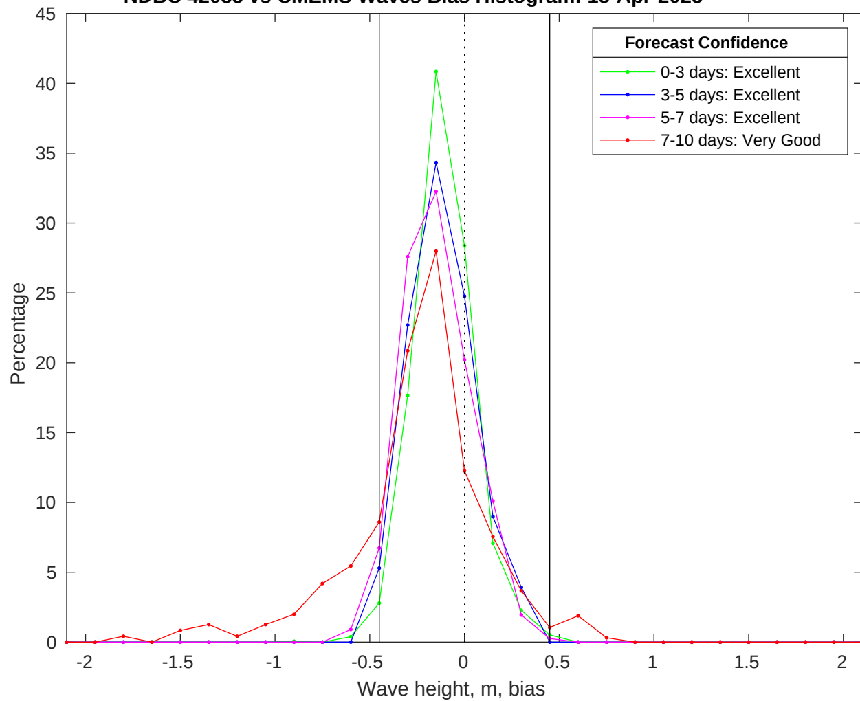
NDBC 42035 vs CMEMS Waves Bias Histogram: 15-Apr-2025
