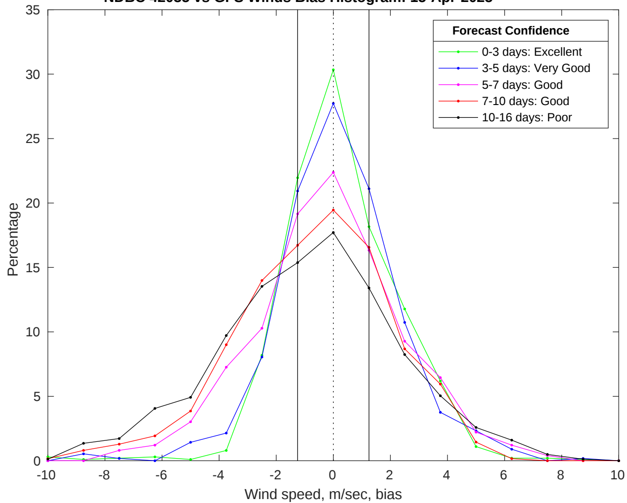
NDBC 42035 vs GFS Winds Bias Histogram: 15-Apr-2025
